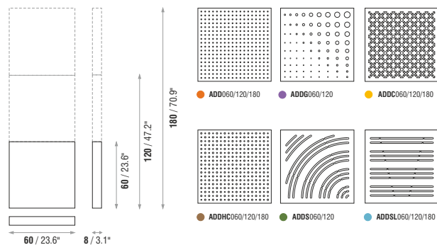
Image of 60x60cm model Ref.:ADD060 (on the left) and Ref.:ADD060 (ambient image).
