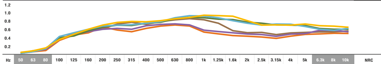
• Values in accordance with the standards: EN 20654, ASTM C423 and EN 11654. ■ Values [ <100\text{Hz} and >5\text{K} ] are Non Standard Values.
